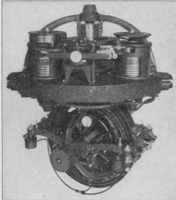
Sensitive Element of Sperry Gyrocompass, Mark X (removed from binnacle).
